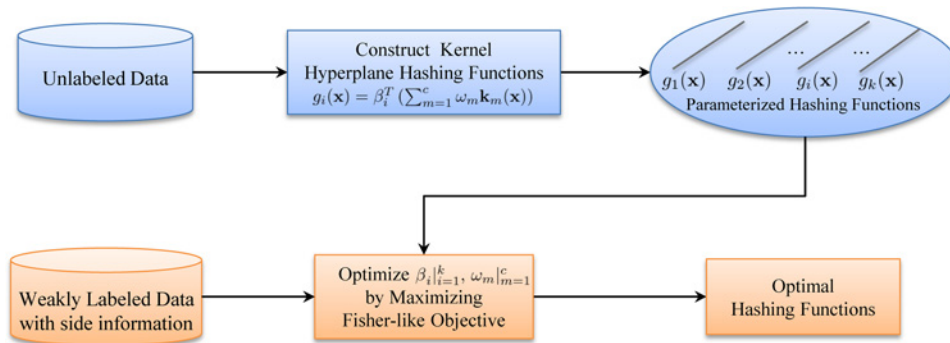
Fig. 1. Overview of the proposed semisupervised hashing method via kernel hyperplane learning (SKHL). In SKHL, each hashing function h_i(\mathbf{x}) (based on g_i(\mathbf{x}) ) is modeled as a nonlinear kernel hyperplane, which is constructed from an unlabeled dataset, and parameterized by \beta_i . Based on these parameterized hashing functions, the hashing codes of the samples from the weakly labeled data set are used to formulate a Fisher-like objective function, which is maximized to learn the optimal hashing functions.
