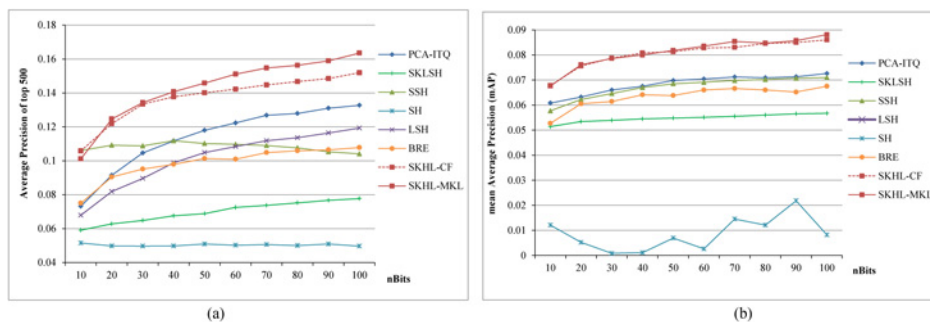
Fig. 2. Results of different methods on the CIFAR-100 dataset in terms of (a) average precision of top 500 and (b) mean average precision (mAP).
