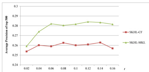
Fig. 9. Performance variations of our SKHL-CF and SKHL-MKL with different parameter t on the NUS-WIDE dataset.
