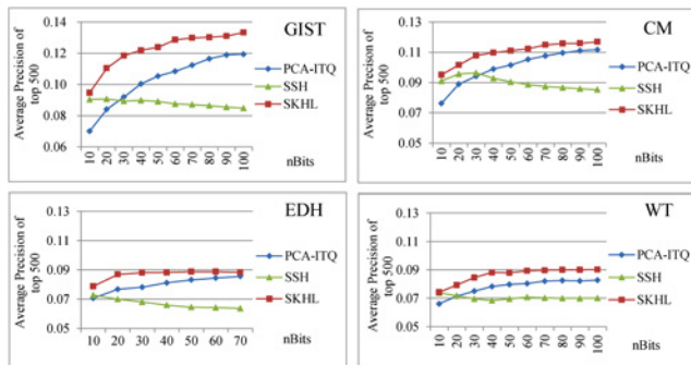
Fig. 7. Comparison between our method SKHL and two most competitive methods PCA-ITQ and SSH when using each type of feature (i.e., GIST, CM, EDH, or WT) on the CIFAR-100 dataset.
