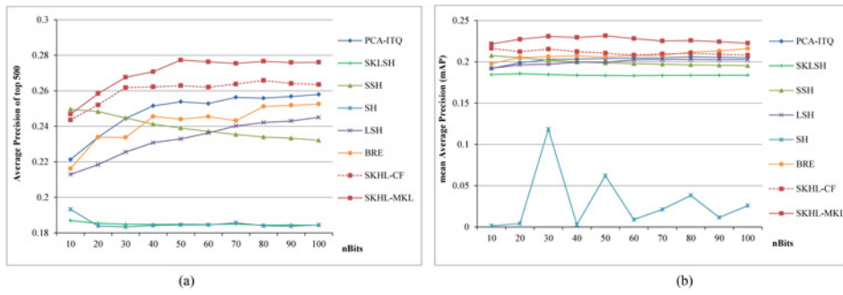
Fig. 4. Results of different methods on the NUS-WIDE dataset in terms of (a) average precision of top 500 and (b) mean average precision (mAP).
