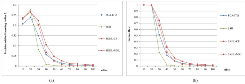
Fig. 5. Comparison of our methods SKHL-CF and SKHL-MKL with two most competitive methods PCA-ITQ and SSH on the NUS-WIDE dataset in terms of (a) precision within Hamming radius 2 and (b) success rate.
