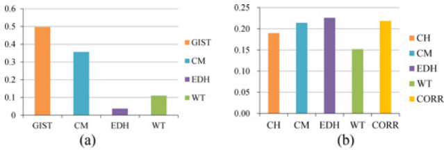
Fig. 6. Learnt weights for each type of feature from our SKHL-MKL on two datasets. (a) CIFAR-100 dataset. (b) NUS-WIDE dataset.
