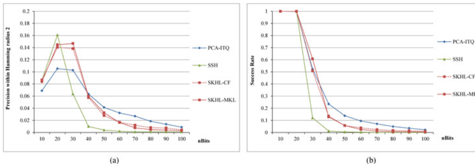
Fig. 3. Comparison of our methods SKHL-CF and SKHL-MKL with two most competitive methods PCA-ITQ and SSH on the CIFAR-100 dataset in terms of (a) precision within Hamming radius 2 and (b) success rate.
