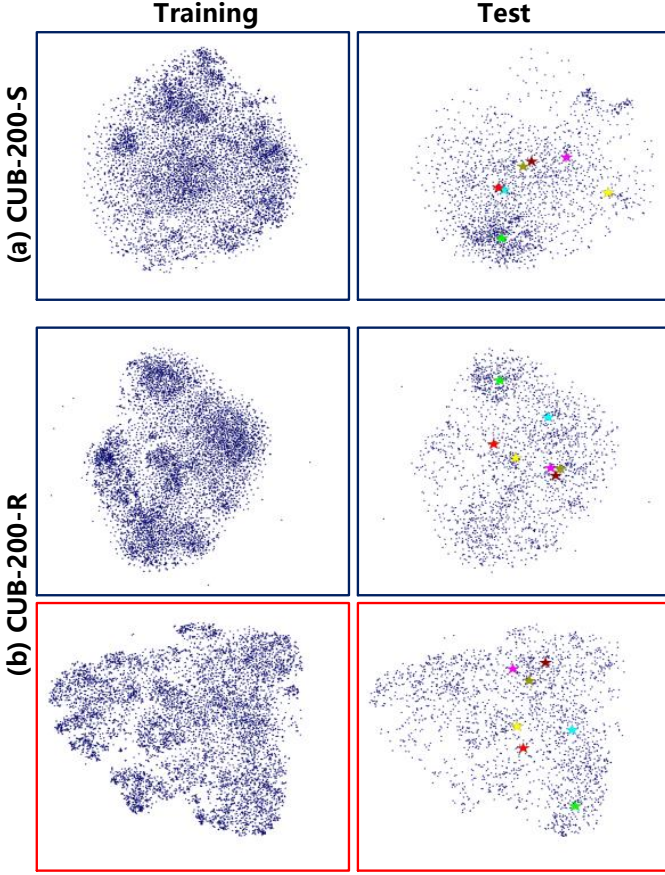
Fig. 3: The visualization of image representations of all training and test categories on CUB-200-S and CUB-200-R using t-SNE [55]. Each image is visualized as one point. The scatter plots in blue and red boxes come from OFL and AGFL, respectively. In test categories, the centers of some categories are represented by pentagrams of different colors, and the pentagram of same color represents the same category across different datasets or methods.
