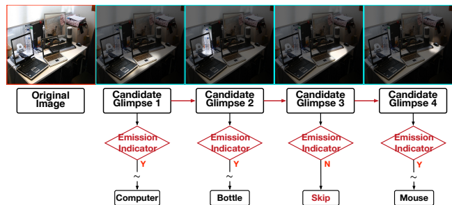
Figure 1: The RHN generates a sequence of candidate glimpses which can highlight the specific regions, and the emission indicator adaptively select which glimpse should be emitted to the real prediction set for further label relation modeling and classification.
