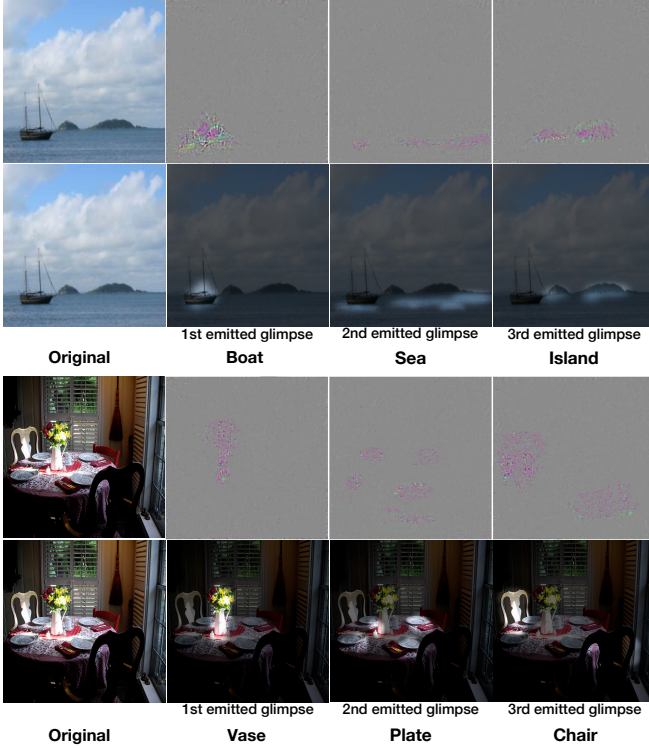
Figure 6: Visualization of regions with high activations at different emitted glimpses. The first column is the original image, and the rest are the high activation maps and corresponding highlighted multi-label images.
