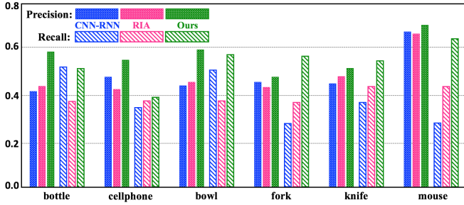
Figure 5: Comparison performances on small objects between CNN-RNN [36], RIA [14] and Ours.
