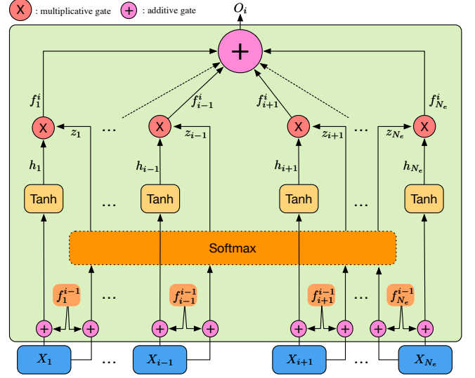
Figure 4: The unit of GRRE at the i th emitted glimpse. It models the label relation from all other emitted glimpses to the i th emitted glimpse.
