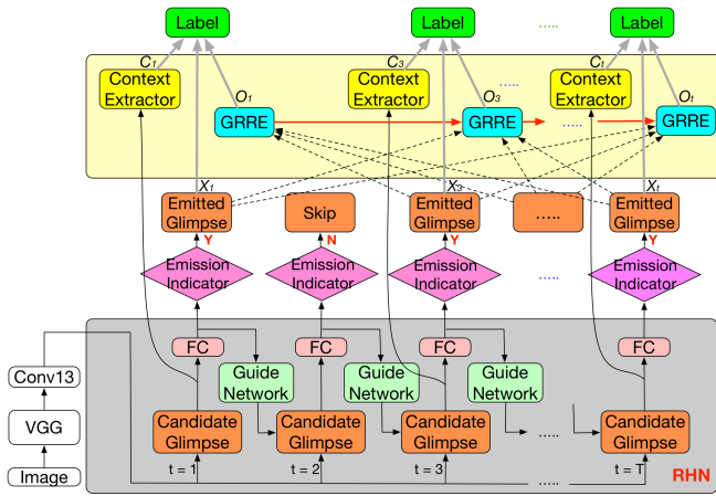
Figure 2: Main architecture of the proposed attentive recurrent neural network. The input image is fed into VGG16 to extract features from the last convolutional layer. Then RHN generates a sequence of candidate glimpses based on the guide network. After that, the emission indicator is learned to decide whether the candidate glimpse should be emitted. The emitted glimpses are sent into the proposed GRRE to model the label relations. Finally, the label is predicted based on three parts, i.e., the features from emitted glimpses, the context features extracted from emitted glimpses via the context extractor, and the label relations from GRRE.
