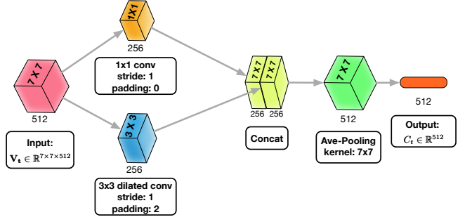
Figure 3: Illustration of the context extractor
