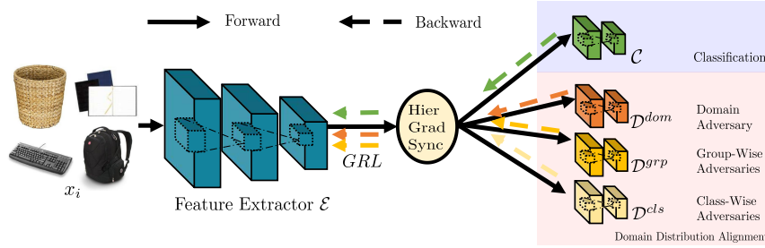
Figure 2. Illustration of the overall framework of our GSDA method. An input sample x_i from source or target domain is firstly encoded by the common feature extractor \mathcal{E} . Based on the extracted feature, the classifier \mathcal{C} is designed for object classification, and the adversarial discriminators including \mathcal{D}^{dom} , \mathcal{D}^{grp} and \mathcal{D}^{cls} are designed for distribution alignment from perspective of domain-level, group-level and category-level respectively. Furthermore, a hierarchical gradient synchronization between the three types of adversarial discriminators is constructed to constrain the consistency between global and local alignment for better structure preservation. Best viewed in color.
