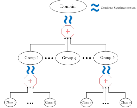
Figure 3. Illustration of the hierarchical distribution alignments and hierarchical gradient synchronization among them.
