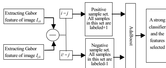
Fig.4. Framework of the proposed training process.
