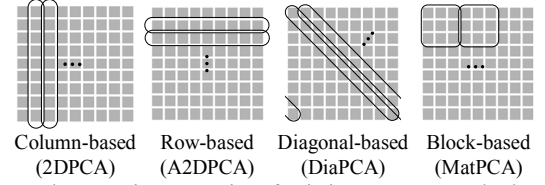
Fig.1. The grouping strategies of existing 2D PCA methods. The grey panes represent an enlarged 9 \times 9 face image matrix, each pane corresponding to a pixel (a random variable) in the image. The panes in a round rectangle constitute a group.
