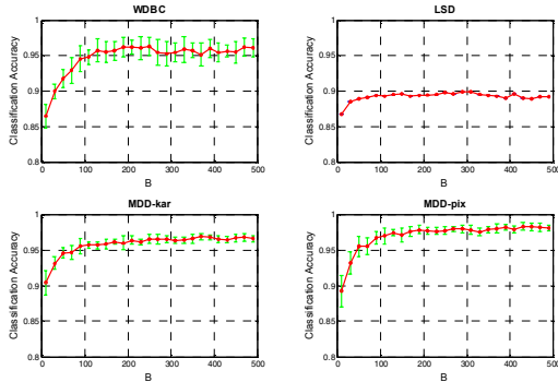
Fig.8. Effect of different parameters B on classification accuracy when K equals to 10. Means (red) and standard deviations (green) of classification accuracies are given.
