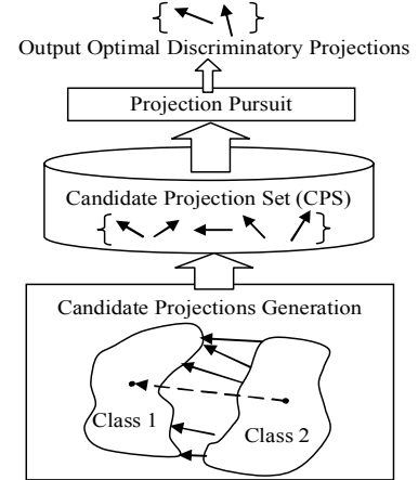
Fig.1. Proposed paradigm for linear feature extraction.
