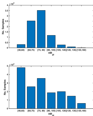
Fig. 7. The ground-truth HR distribution (top) and the augmented HR distribution (bottom) of the VIPL-HR database [13].
