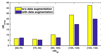
Fig. 11. The estimation error ( HR_{r,mse} ) of videos with ground-truth HRs in different HR ranges for the method with and without our data augmentation module.
