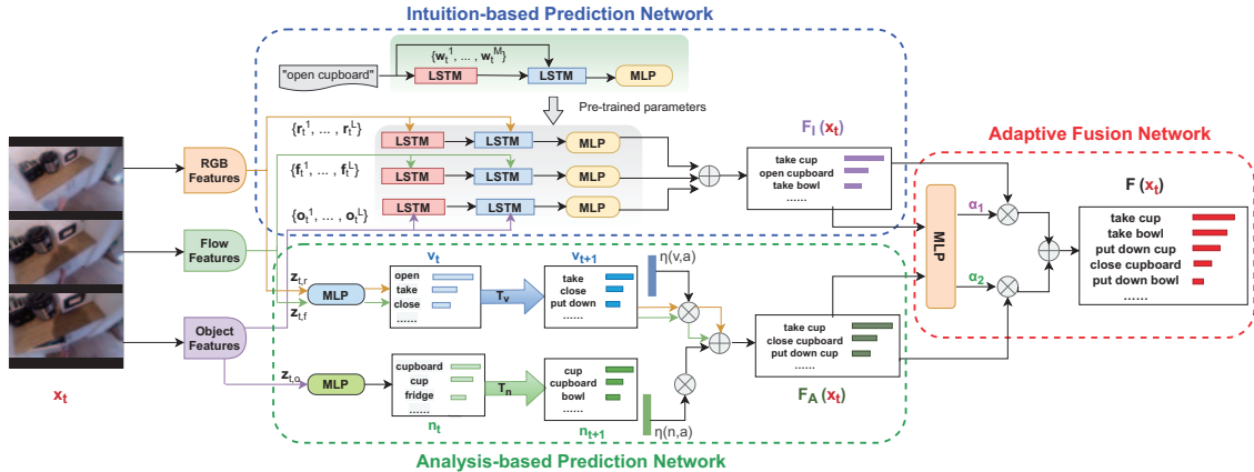
Figure 3: The concrete architecture of our IAI framework where the three sub-networks are explicitly modeled. Given x_t , outputs from IPN and APN (i.e., F_I(x_t) and F_A(x_t) ) are integrated to obtain the final anticipation result F(x_t) via AFN.
