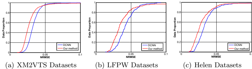
Fig. 9. Comparison with DCNN [26]
